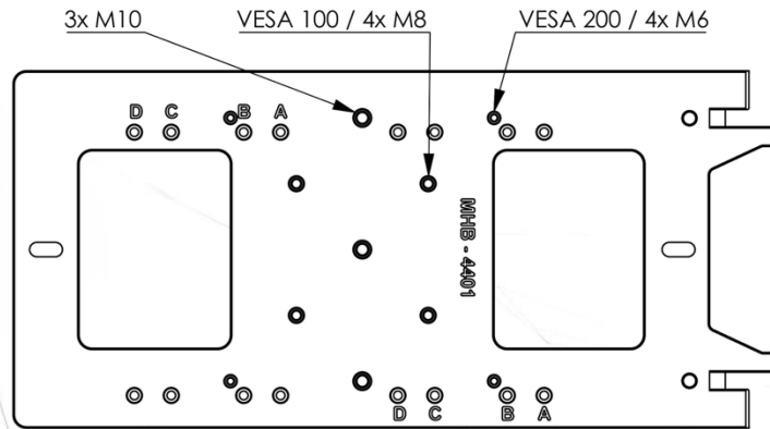
Projector Plate MHB-4401 for the Barco i600 projectors
