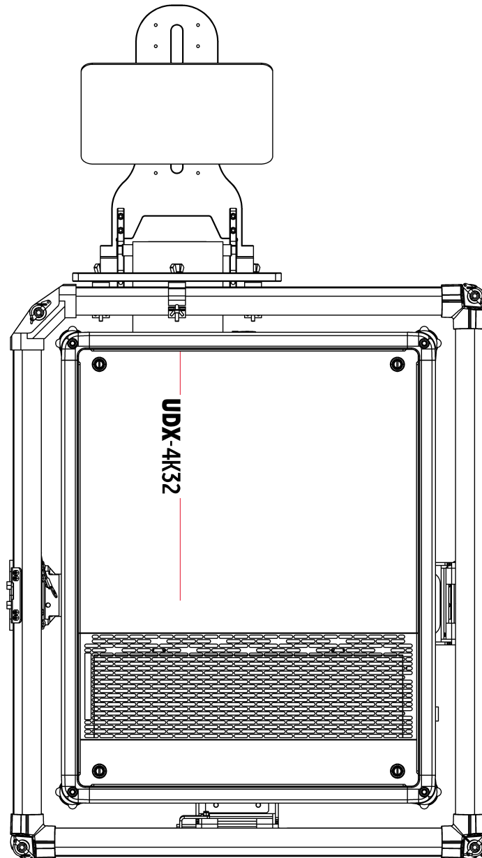
Barco UDX-4K32 with TLD + 1.5-2.0:1 (1.49-2.03:1 4KUHD) + ULS Mirror M340
